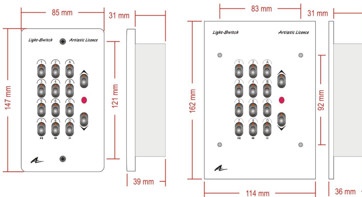
Mounting Drawing
