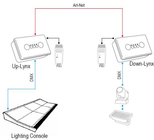
Application Drawing
