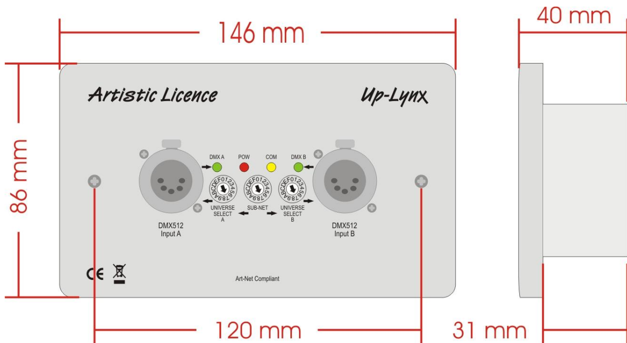
Mounting Drawing
