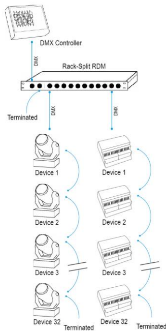
Single DMX Splitter - Recommended Arrangement
