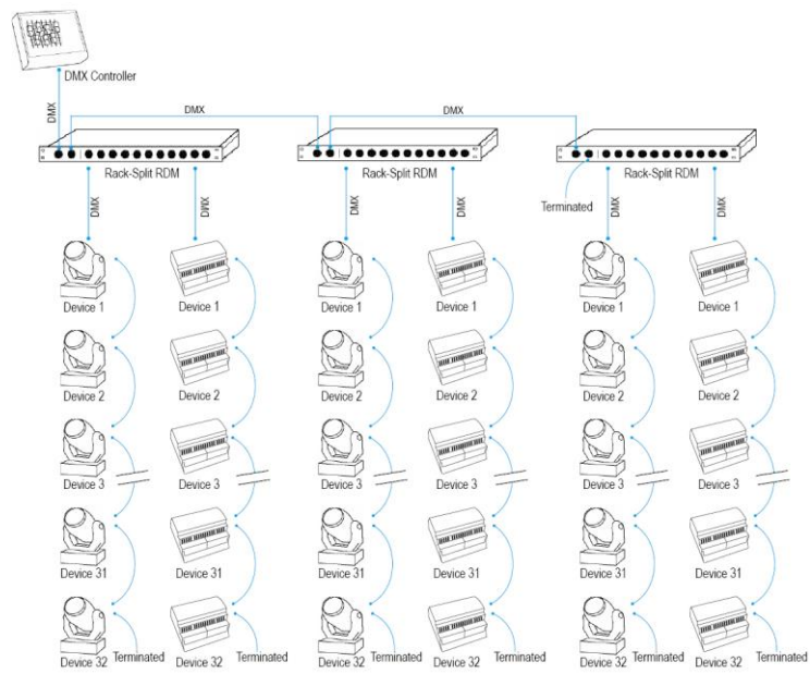
Multiple DMX Splitters - Recommended Arrangement
